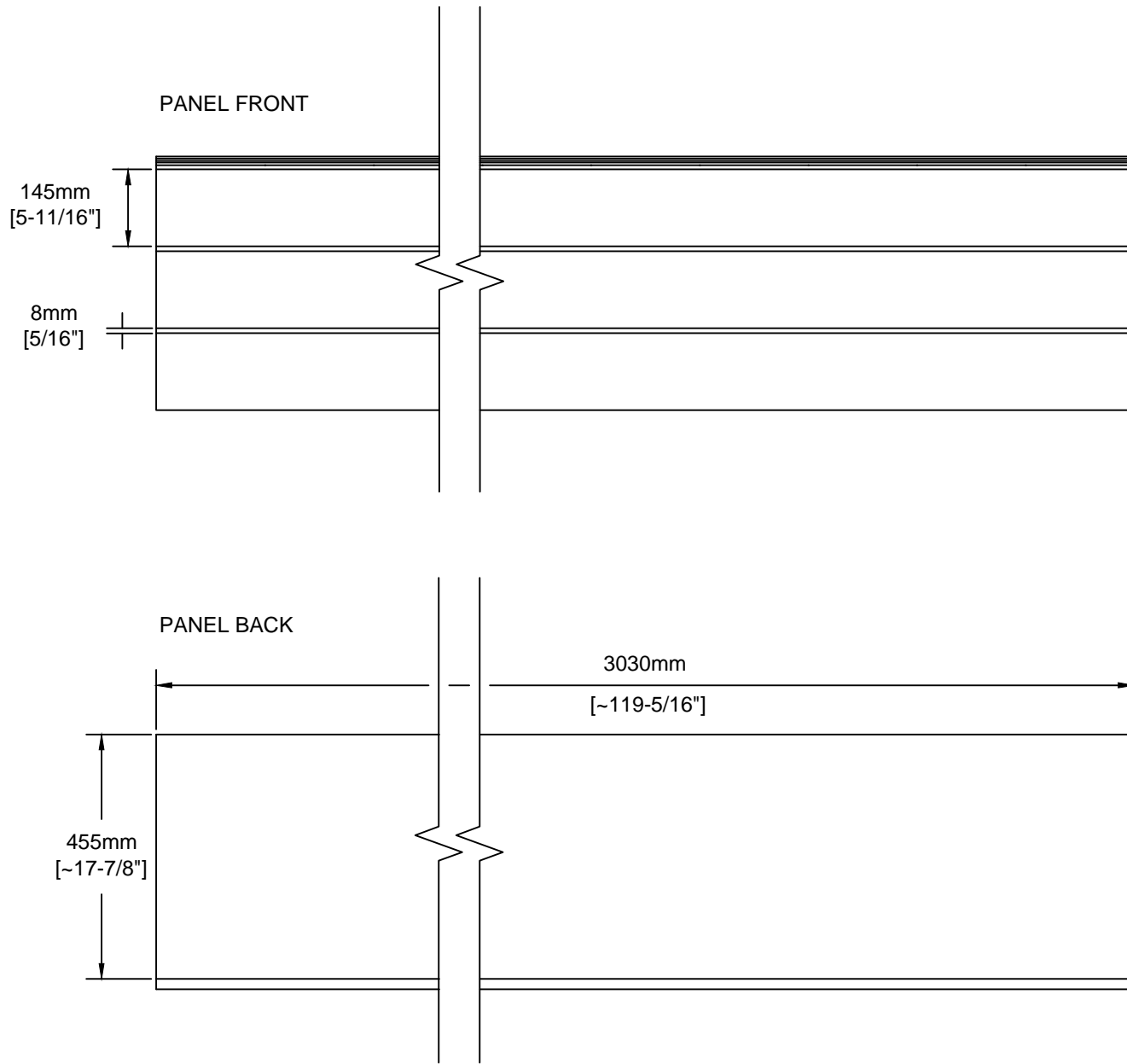
AWP-3030 - VINTAGE WOOD PANEL DETAIL SCALE: 1" = 1'-0"
