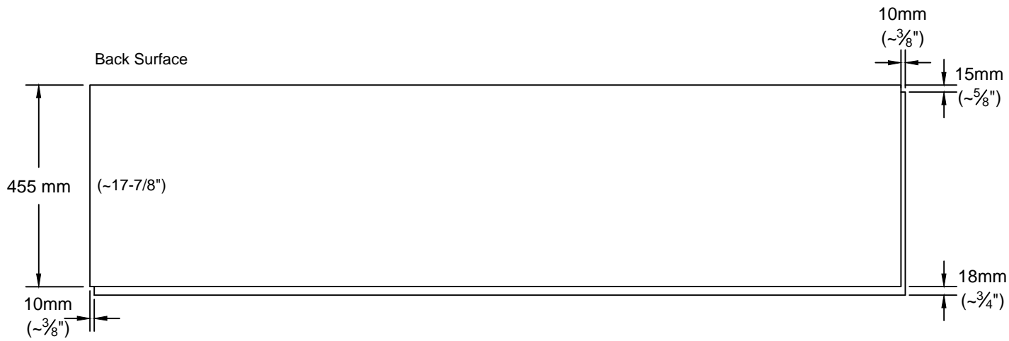
NICHIHA VINTAGEWOOD 1818 PANEL DETAIL SCALE: 1" = 1'-0"
