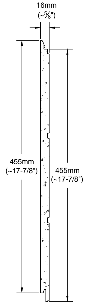
PANEL SECTION
