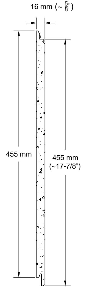
PANEL SECTION
