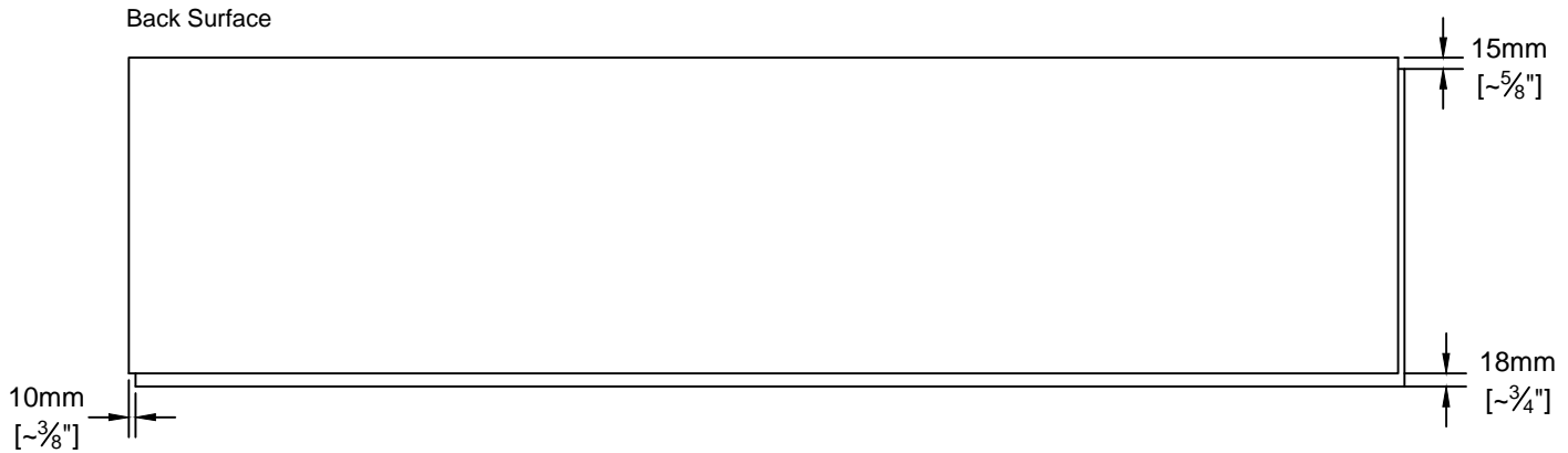
AWP-1818 - SANDSTONE PANEL DETAIL SCALE: 1" = 1'-0"
