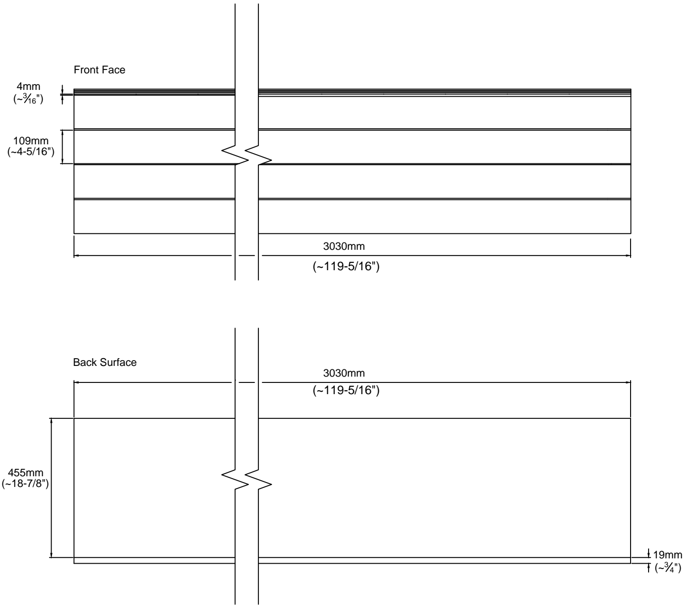
AWP-3030 - ROUGHSAWN - PANEL DETAIL SCALE: 1" = 1'-0"
