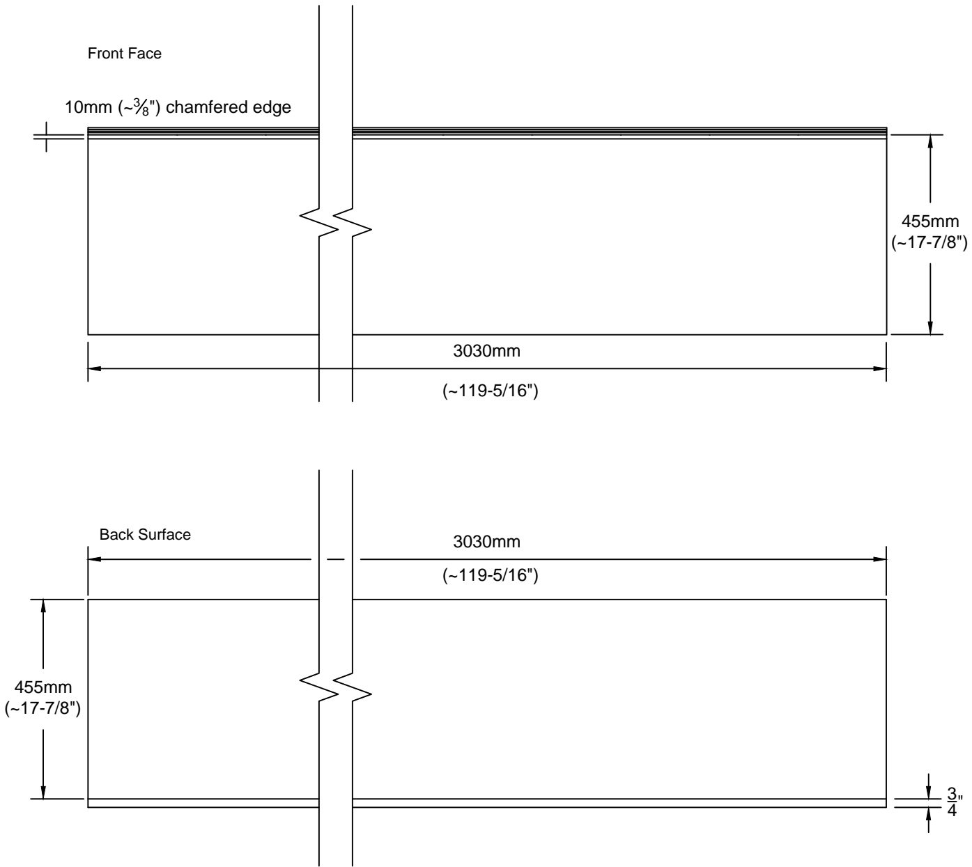
AWP3030 - INDUSTRIAL BLOCK PANEL DETAIL SCALE: 1" = 1'-0"
