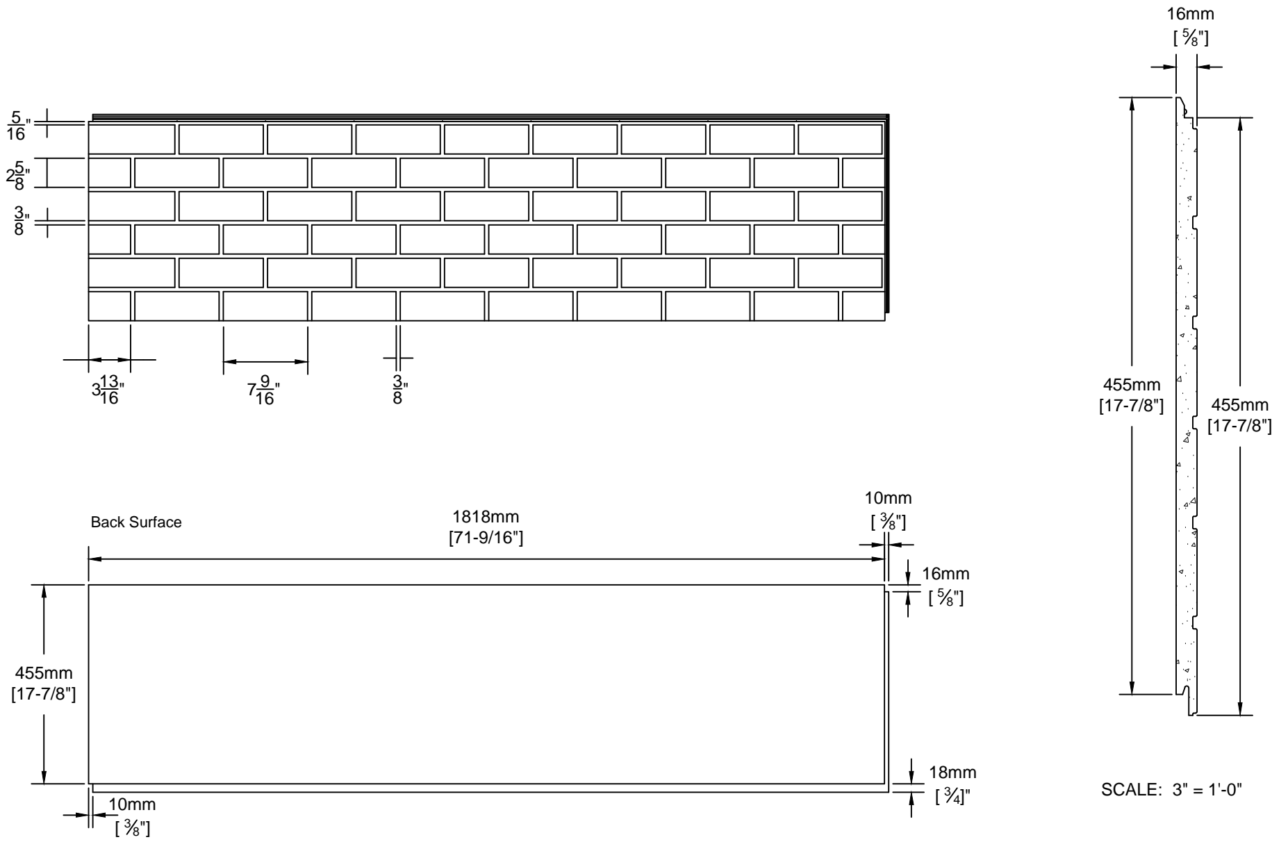
CANYON BRICK PANEL DETAIL SCALE: 1" = 1'-0"
