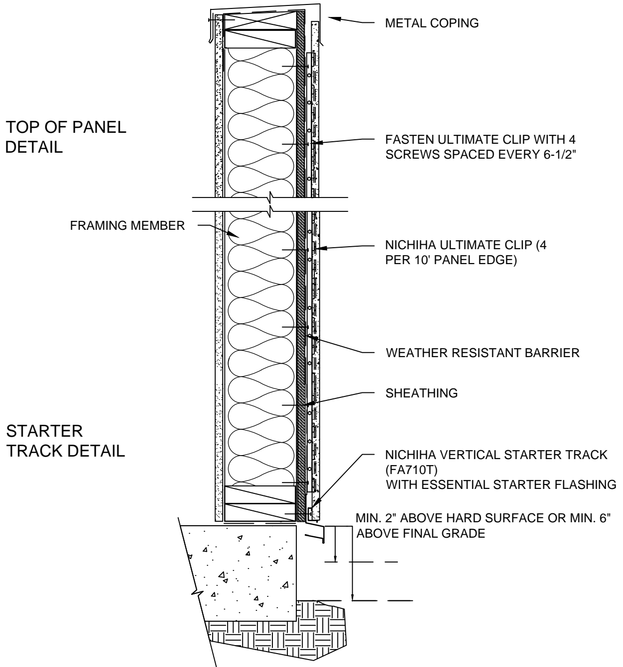
NICHIIHA VERTICAL AWP - 3030 - TYPICAL WALL SECTION - PARAPET
