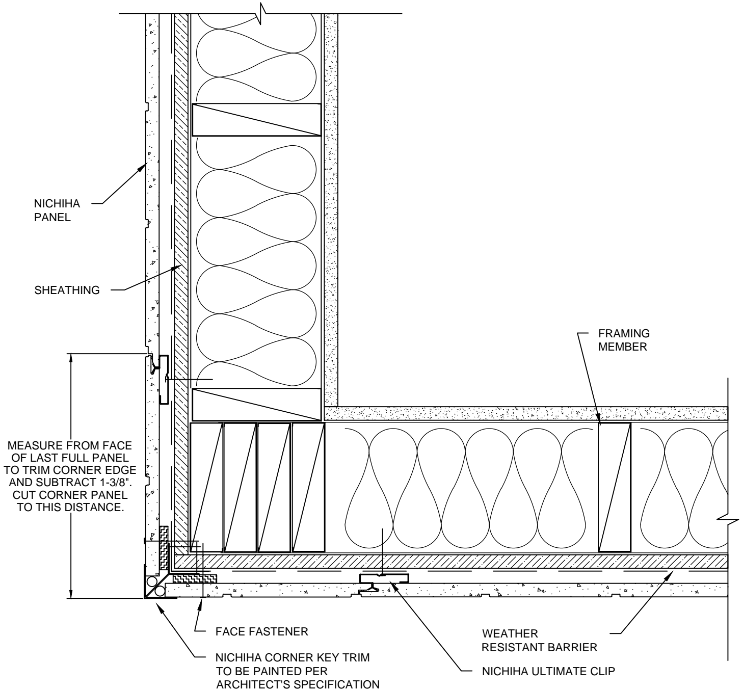
NICHIIHA AWP-3030 VERTICAL - OUTSIDE CORNER DETAIL - CORNER KEY TRIM
