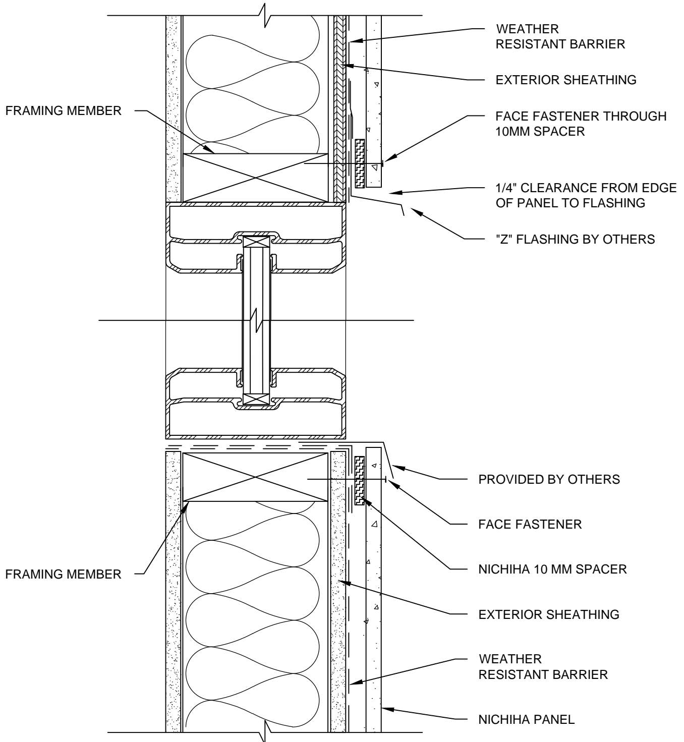
NICHHA HORIZONTAL AWP - RECESSED WINDOW - HEADER & SILL WITH FLASHING
