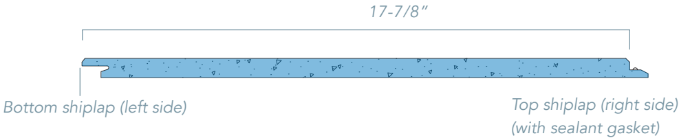
PANEL SECTION (PLAN VIEW)
